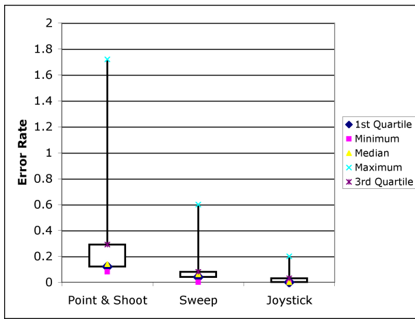
Figure 6. Error rates for multidirectional tapping test grouped by input technique.
