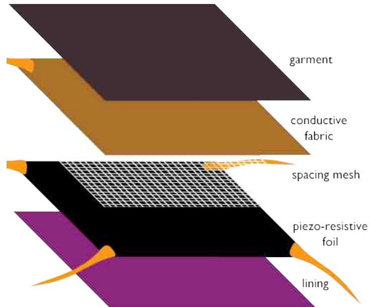
Figure 4.1: Initial layered architecture. The three layers in the middle allow sensing touch and determining its location.
