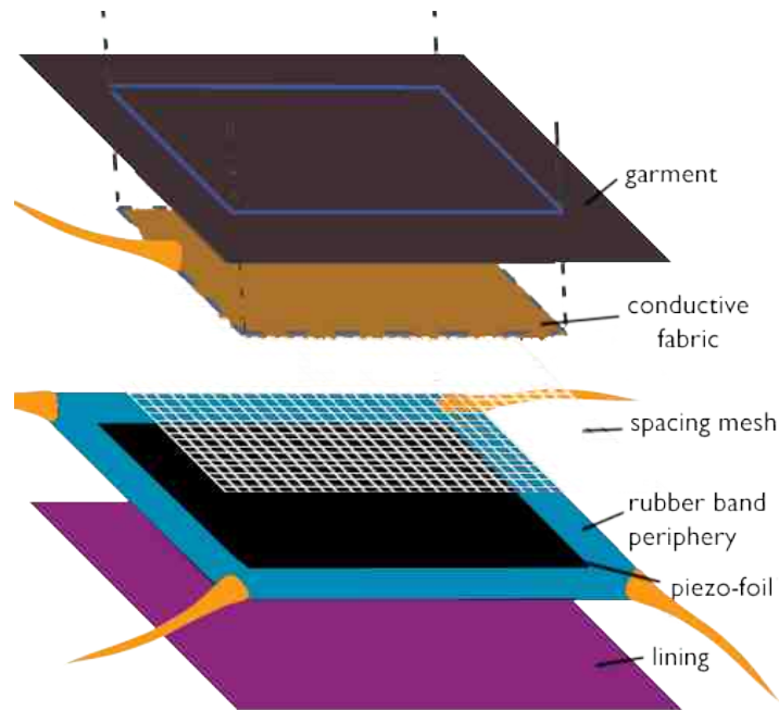
Figure 4.3: Improved layered architecture. Conductive fabric is removed in periphery area of the sensor and replaced by a rubber outline.
