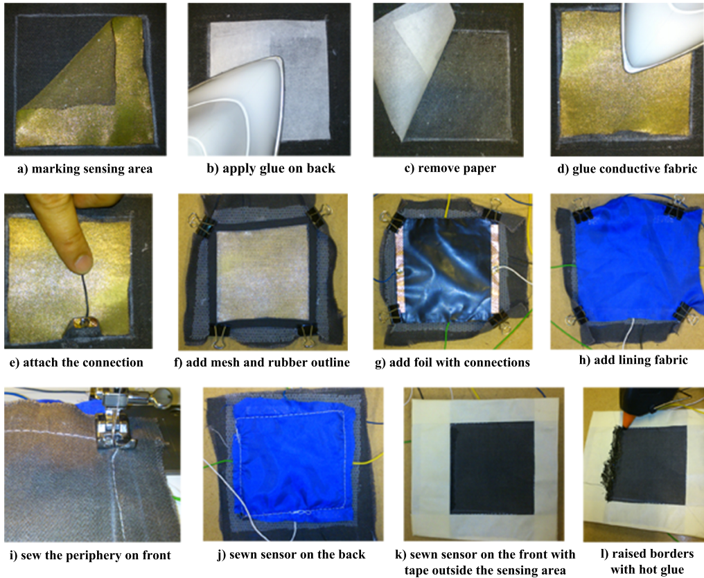
Figure 5.1: Steps for creating TextiPad . a) to e) depict adding the first layer, f) to h) the other ones, and the remaining steps are the finishing procedures.
