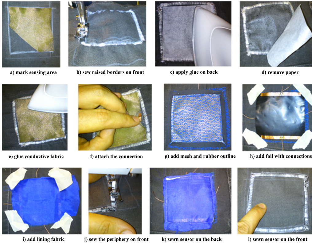
Figure 5.3: Steps for embedding a sensor in GestiPants . The difference with TextiPad is that sensor borders are done in the very beginning - step b), and the trousers' fabric replaces the textile patch used there.
