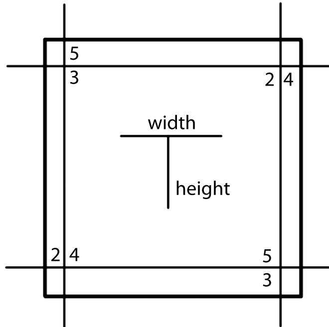
Figure 4.8: Scheme for calibrating the sensor. Two values for each border are extracted and consequently width and height can be computed.
