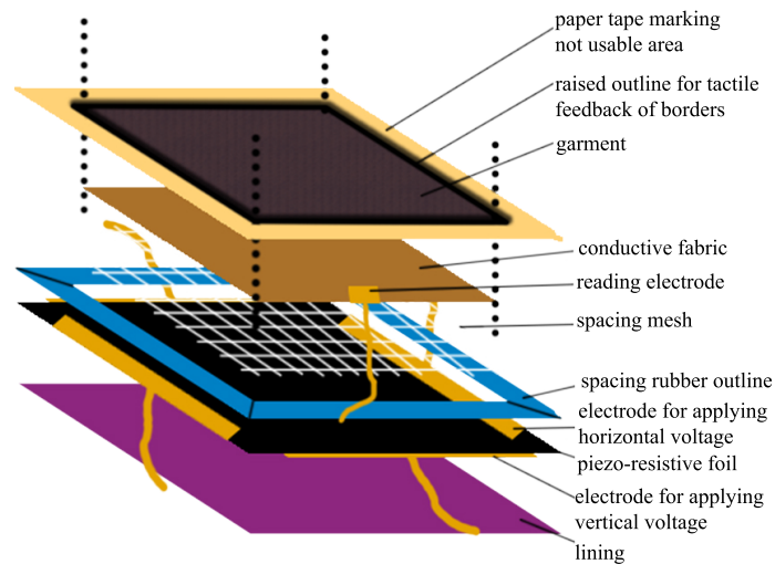
Figure 4.5: Final layered architecture. Electrodes are not placed in the corners anymore, but along the sides of the piezo-resistive layer.
