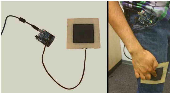
Figure 5.2: Finished prototype ready for evaluation. Left image shows the bare prototype and the right one - its attachment to the right leg of the wearer's jeans.
