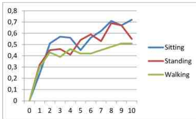
Figure 6.14: Learning curves for all treatments for Gesti-Pants . Sitting condition has the steepest curve, suggesting that users grasp the interaction faster while sitting.
