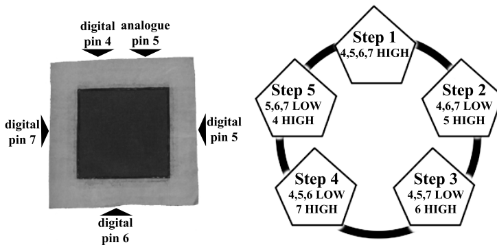
Figure 4.7: Measurement algorithm executed in the beginning of each run loop. On the left is shown the attachment of electrodes to the microcontroller, and on the right - a visualization of the algorithm.
