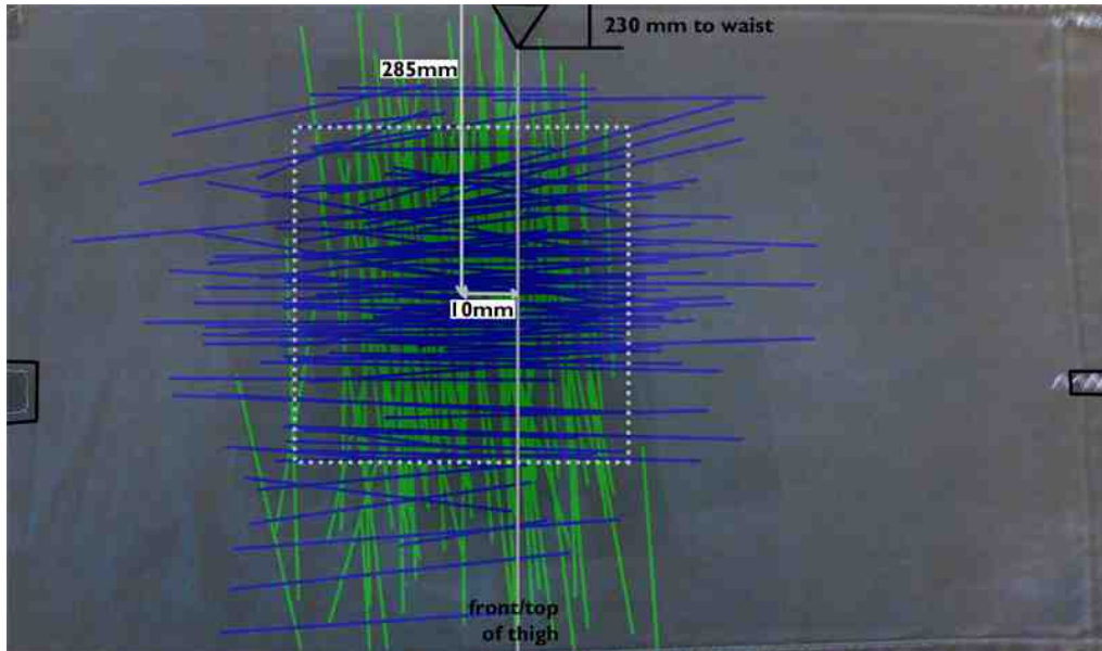
Figure 6.6: Combined placement and orientation map. The image shows that the center of the sensor has to be 285\text{mm} down from the waist and 10\text{mm} away from the top of the thigh towards its outside with vertical borders parallel to the thigh.
